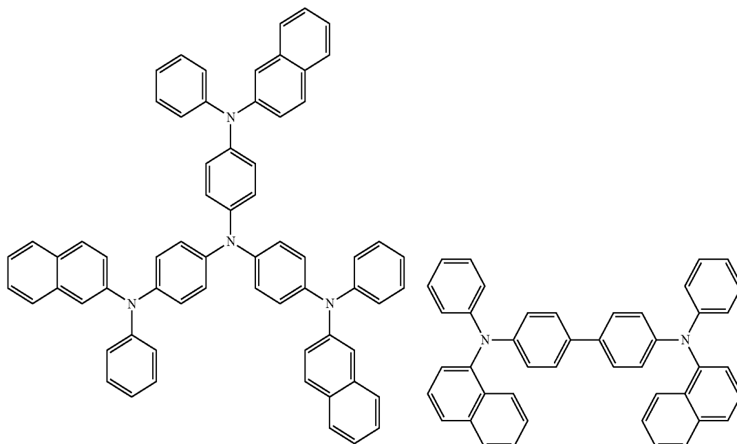
2-TNATA
