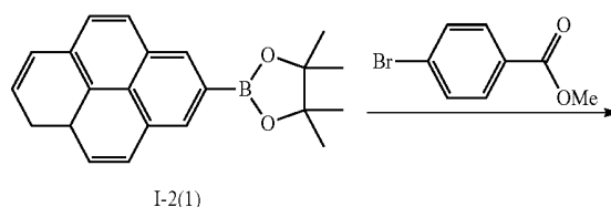
Reaction Scheme 2
