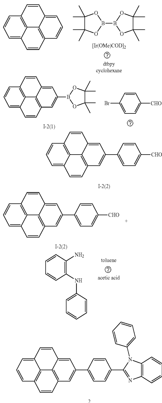
Reaction Scheme 1
