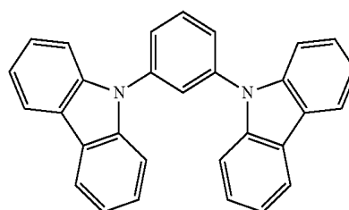
dmCBP
