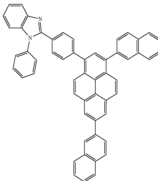
Compound C
